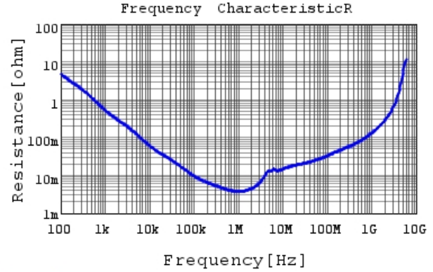
GRM21BR70J106KE76 R DCOV, 25degC
