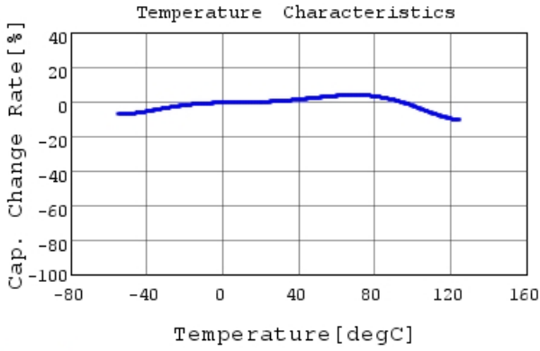
GRM21BR70J106KE76 C-Temp. capchange, DC0.0V,
