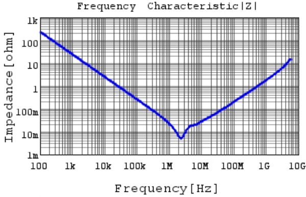
GRM21BR70J106KE76 |Z| DCOV, 25degC
