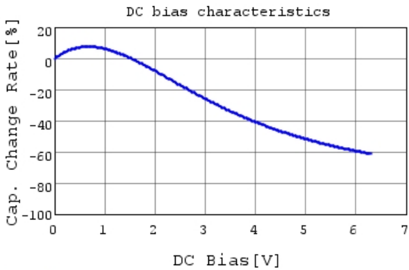
GRM21BR70J106KE76 C-DC bias capchange, 25.0c
