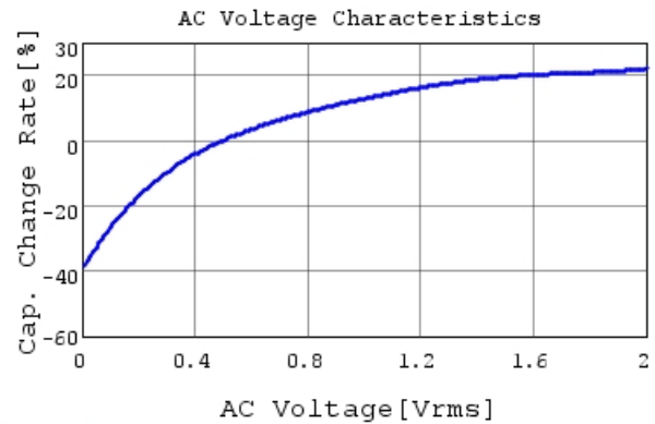
GRM21BR70J106KE76 C-AC Voltage capchange, Dc
