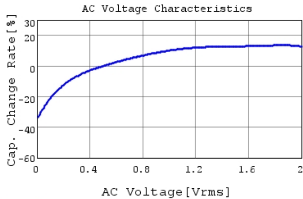
GRM319R61C226ME15 C-AC Voltage capchange, Dc
