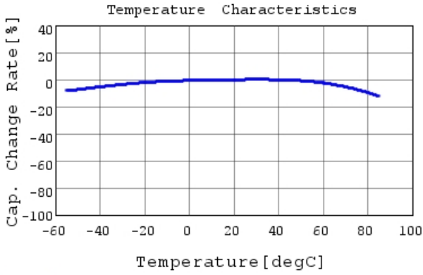
GRM319R61C226ME15 C-Temp. capchange, DC0.0V,
