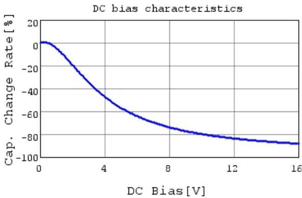
GRM319R61C226ME15 C-DC bias capchange, 25.0c
