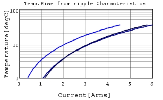
GRM319R61C226ME15 Temp.rise — 80kHz —
