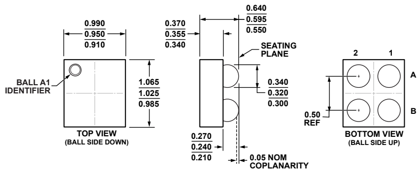
Figure 30. 4-Ball Wafer Level Chip Scale Package [WLCSP] (CB-4-4) Dimensions shown in millimeters
