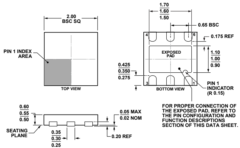
Figure 31. 6-Lead Lead Frame Chip Scale Package [LFCSP_UD] 2.00 x 2.00 mm Body, Ultra Thin, Dual Lead (CP-6-3) Dimensions shown in millimeters
