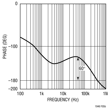
Figure 5. Bode Plot of Figure 1's Circuit
