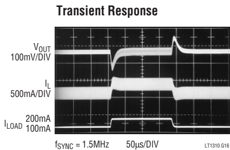
LT1310 G16
