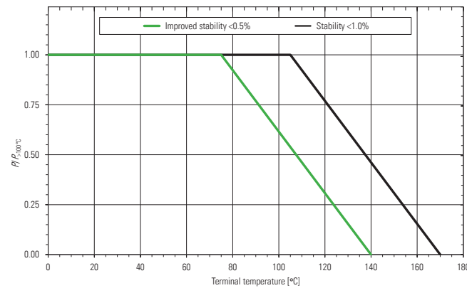
Power derating curve BVS-I-R002 / BVS-I-R003
