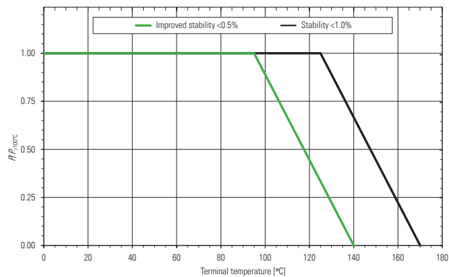
Power derating curve BVS-I-R001
