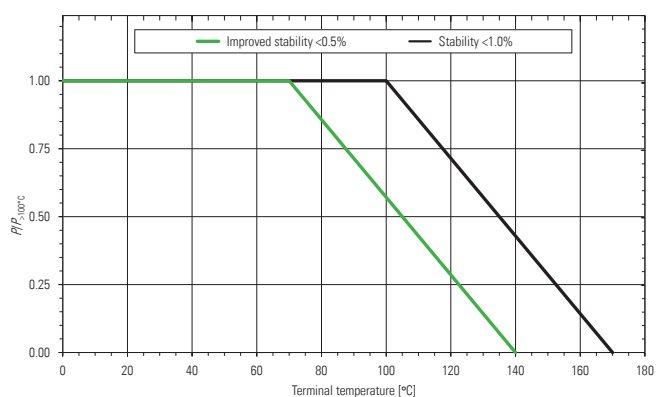
Power derating curve BVS-V-R002 / BVS-I-R004 / R005
